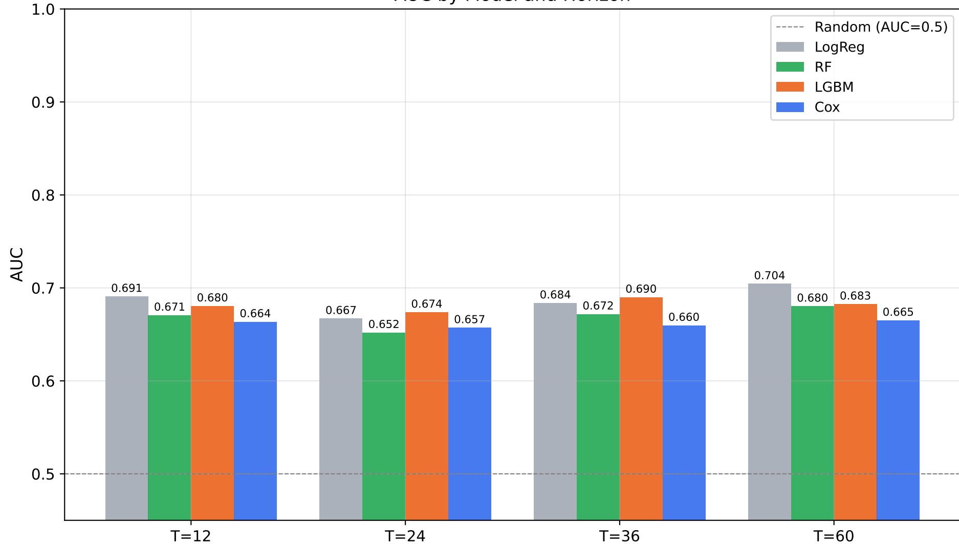
AUC by Model and Horizon
